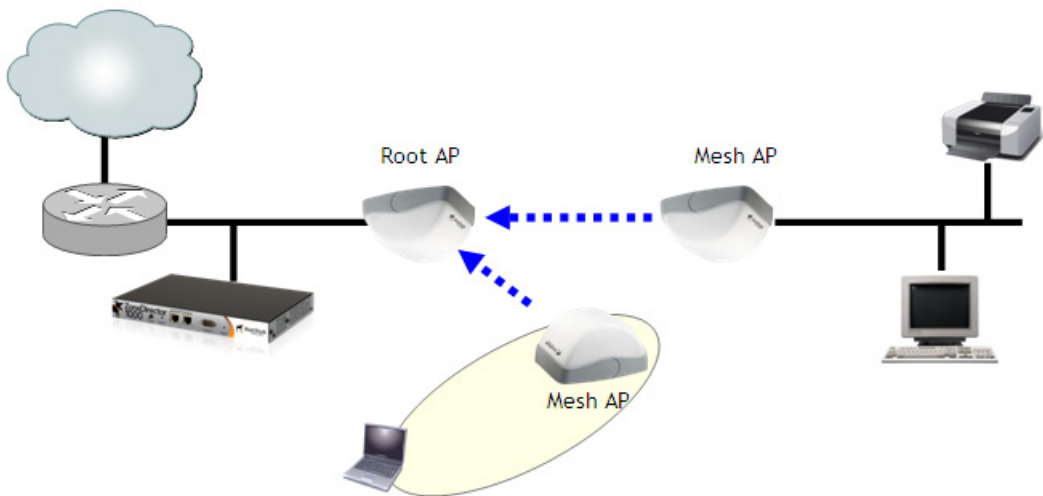
Figure 242. Mesh - wireless bridge topology
