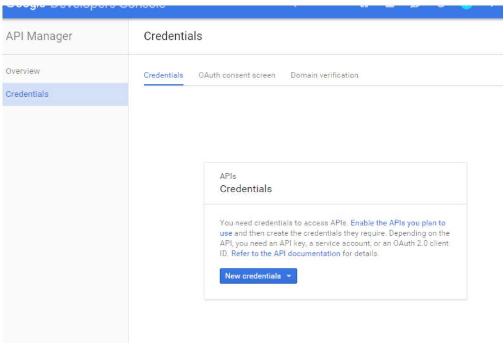
Figure 117. Credentials page
