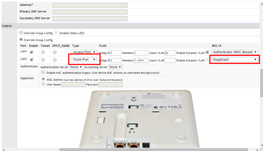
Figure 165. Configuring an AP Ethernet port as an 802.1X Supplicant
