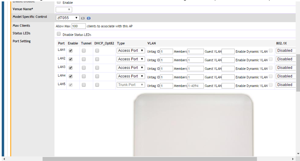
Figure 162. The ZoneFlex 7055 has four front-facing Ethernet ports and one rear port
